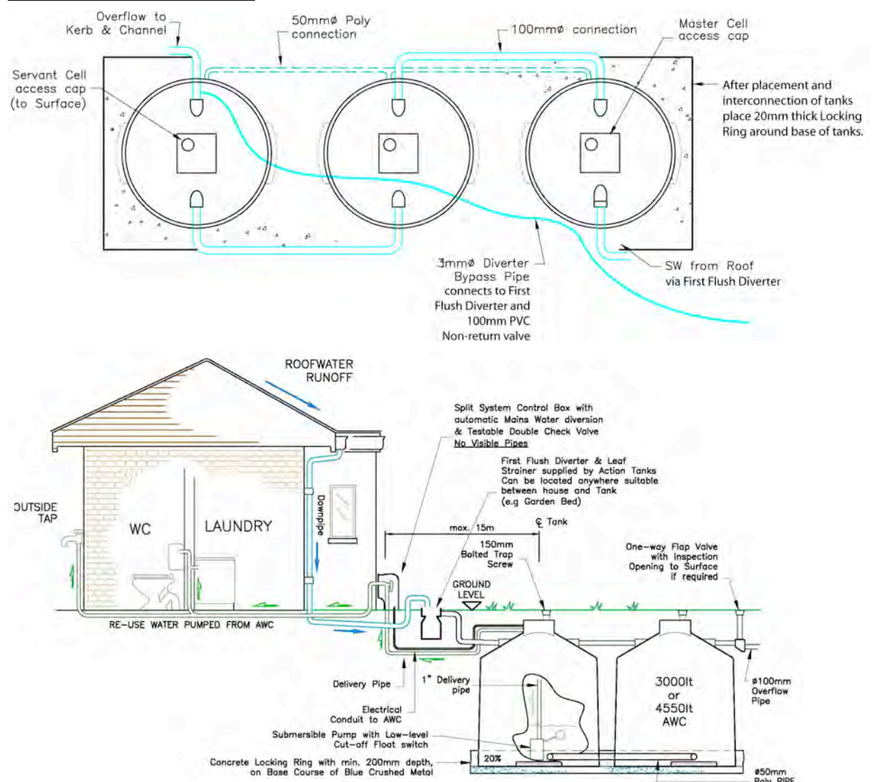
Figure 2: Tank Interconnection
